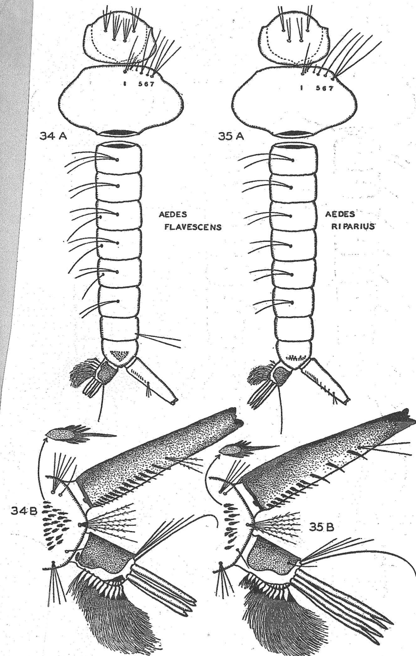
FIGS. 34 AND 35. Larvae of Aedes . A, dorsum of head and thorax, lateral aspect of abdomen; B, terminal abdominal segments enlarged. Inset detail of comb scales.
